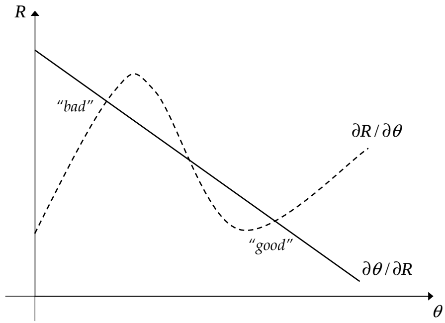
Figure 3. Multiple equilibria
